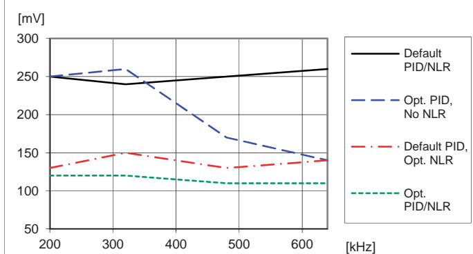
Load transient peak voltage deviation vs. frequency. Step-change (10-30-10 A). T_{P1} = +25\text{ }^\circ\text{C} , V_i = 12\text{ V} , V_0 = 1.0\text{ V} , C_0 = 470\text{ }\mu\text{F}/10\text{ m}\Omega
