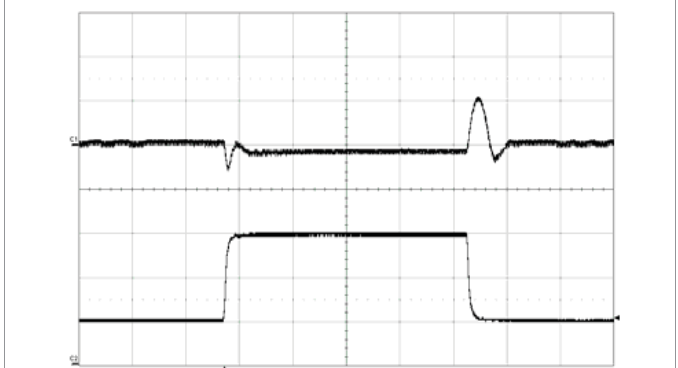
Output voltage response to load current step-change (10-30-10 A) at: T_{P1} = +25\text{ }^\circ\text{C} , V_i = 12\text{ V} , V_0 = 1.0\text{ V} di/dt = 2\text{ A}/\mu\text{s} , f_{sw} = 320\text{ kHz} , C_0 = 470\text{ }\mu\text{F}/10\text{ m}\Omega Top trace: output voltage (200 mV/div.). Bottom trace: load current (10 A/div.). Time scale: (0.1 ms/div.).
