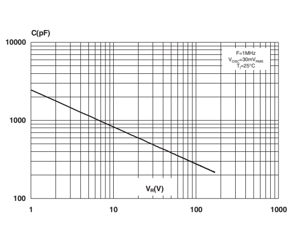
Figure 6. Junction capacitance vs. reverse voltage applied (typical values, per diode)
